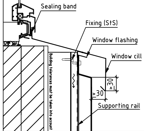
Window horizontal
