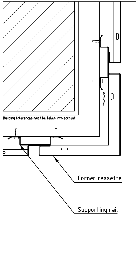
External corner, Alt.1
