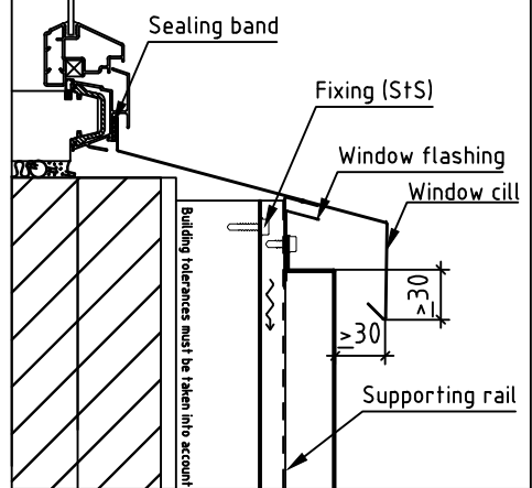
Window horizontal
