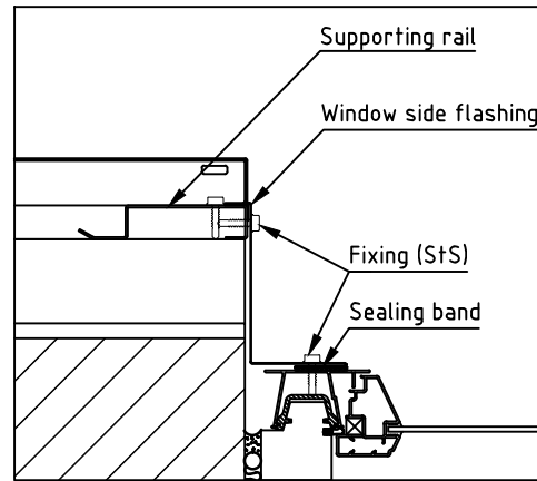
Window vertical
