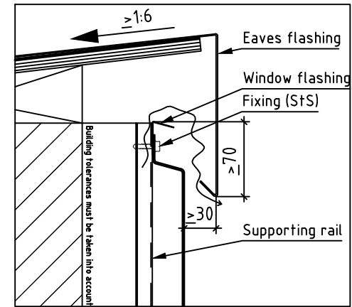
Eaves
