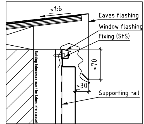
Eaves
