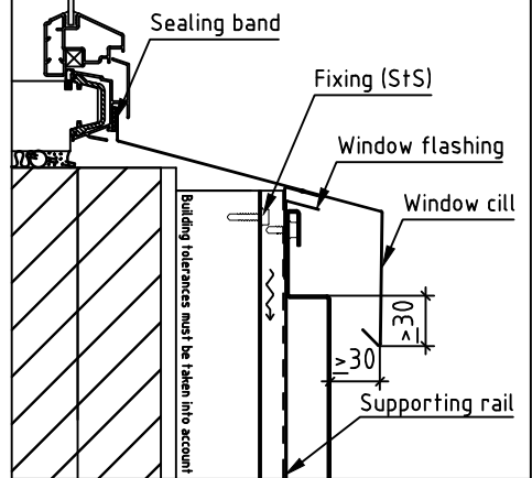
Window horizontal
