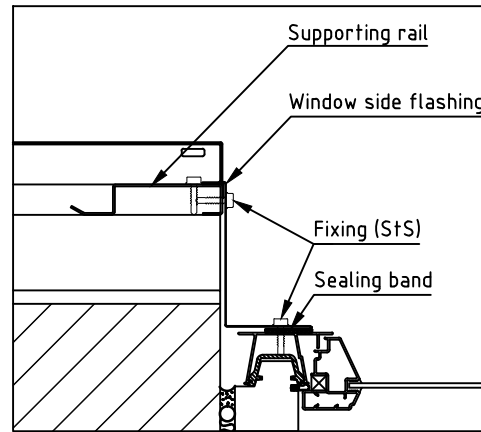
Window vertical
