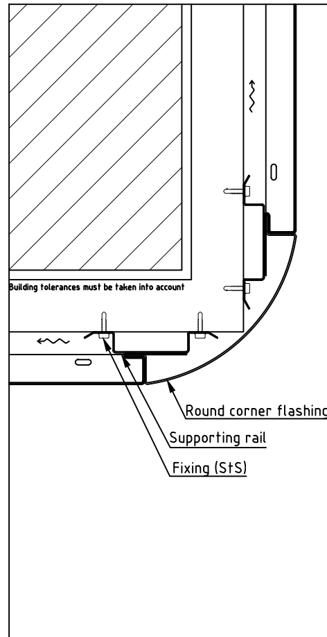
External corner, Alt.2
