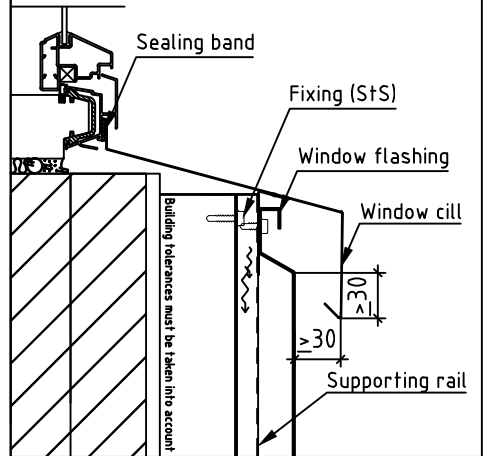
Window horizontal
